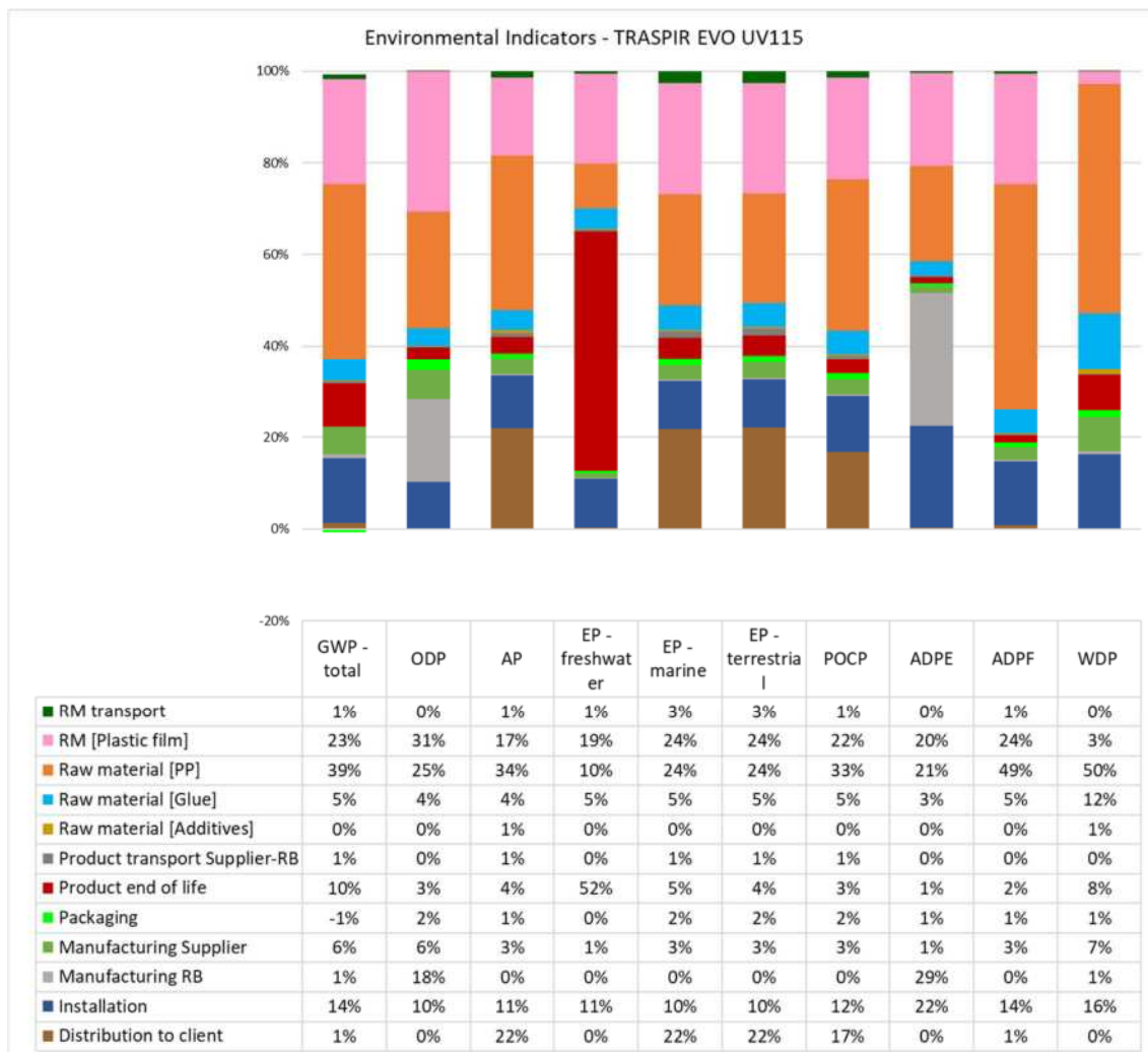
Figure 13. Relative contribution [%] processes-based environmental indicators for TRASPIR EVO UV115
