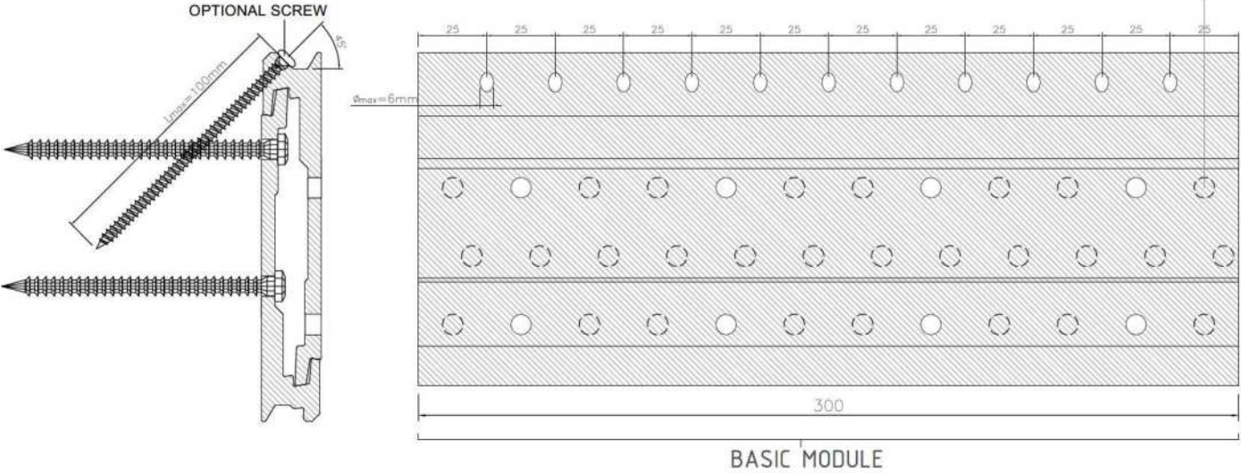
VIEW OF THE CONNECTOR IN THE JOIST
