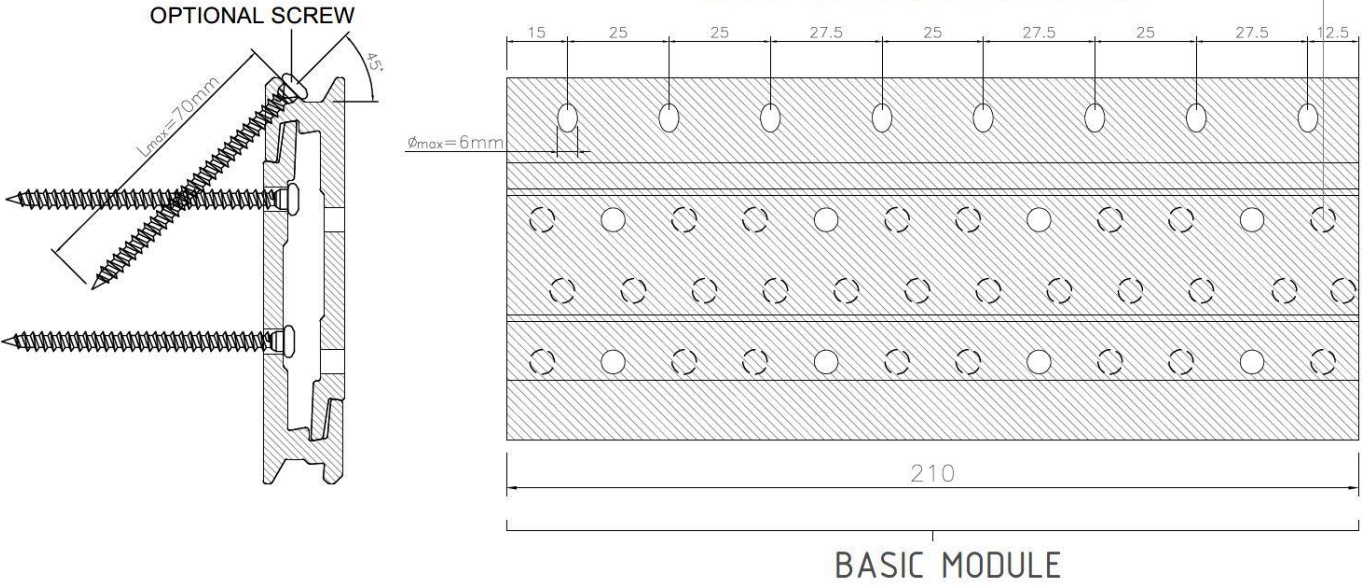
VIEW OF THE CONNECTOR IN THE JOIST
