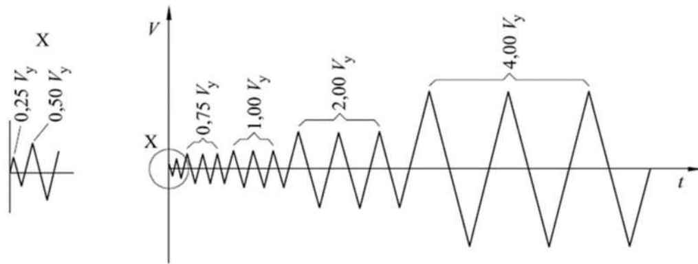
Figure 6. Load steps adopted for the cyclic tests.
