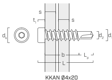
ΚΚΑΝ Ø4x20
