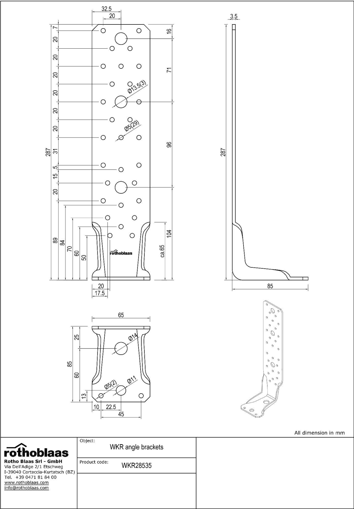
Figure B. 22 Dimensions of Rotho Blaas WKR28535
