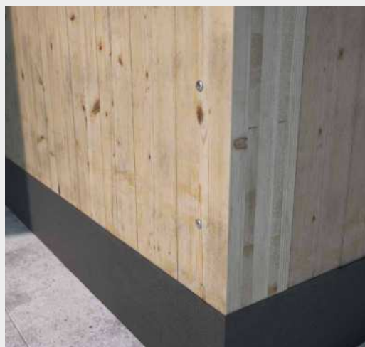
Fixovanie stien z CLT so skrutkami TBS.
